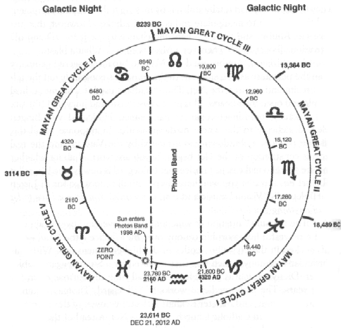
FIGURE 14: THE GREAT STORY OF TIME
