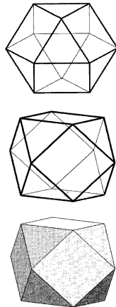
Cuboctaedro
